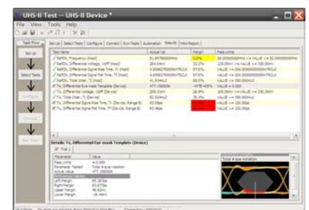
Comprehensive analysis that automates the complex measurements even when you are not there.
