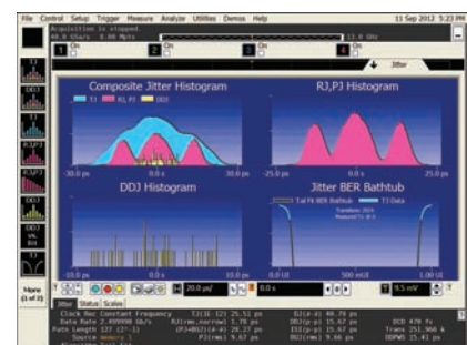
Analyze jitter plus RJ/DJ separation.
