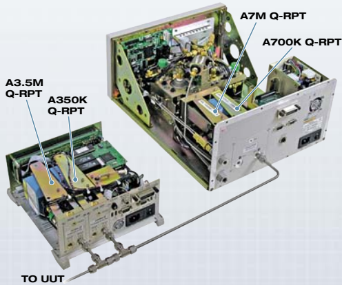
TO UUT PPC4 A7M with RPM4 A3.5Ms/A350Ks
