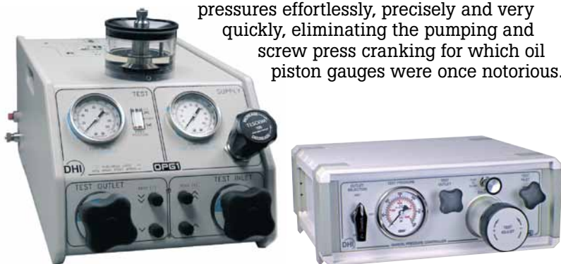
OPG1 Hydraulic Pressure Generator/Controller MPC1 Manual Pressure Controller
