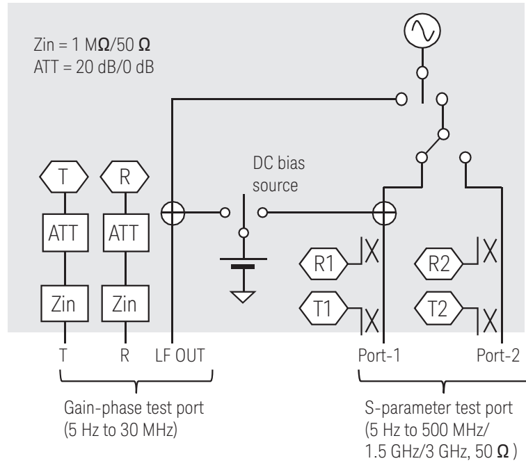
E5061B-3L3/3L4/3L5 block diagram
