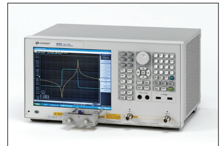
Gain-phase series-thru method using 16047E 4TP fixture
