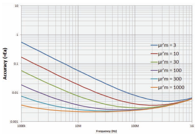
Figure 49. Permeability loss tangent ( \tan\delta ) accuracy vs. frequency (at F = 3 mm, typical) 1
