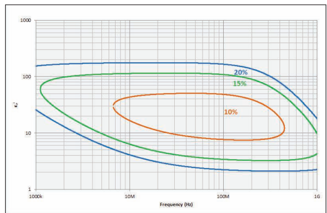
Figure 21. Permittivity ( \epsilon'_\rho ) vs. frequency (at t = 3 mm, typical)
