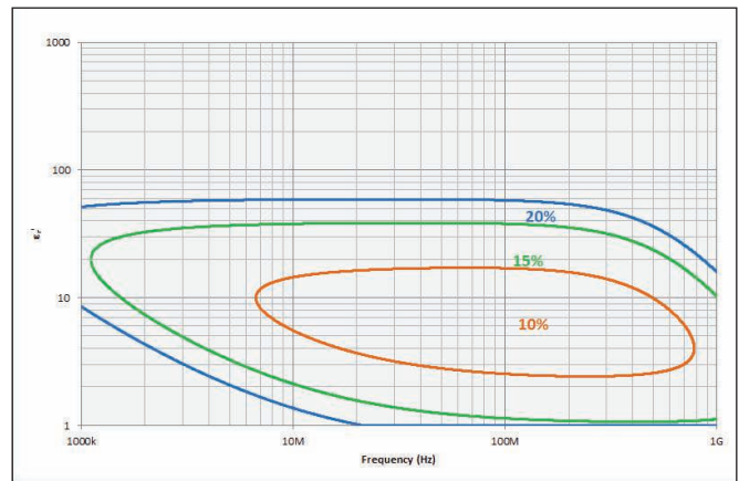
Figure 20. Permittivity ( \epsilon'_\rho ) vs. frequency (at t = 1 mm, typical)
