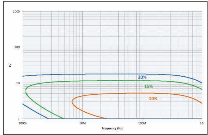
Figure 19. Permittivity ( \epsilon'_\rho ) vs. frequency (at t = 0.3 mm, typical)
