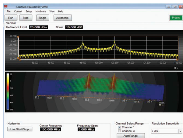
Waterfall view for ASV spectrogram measurement
