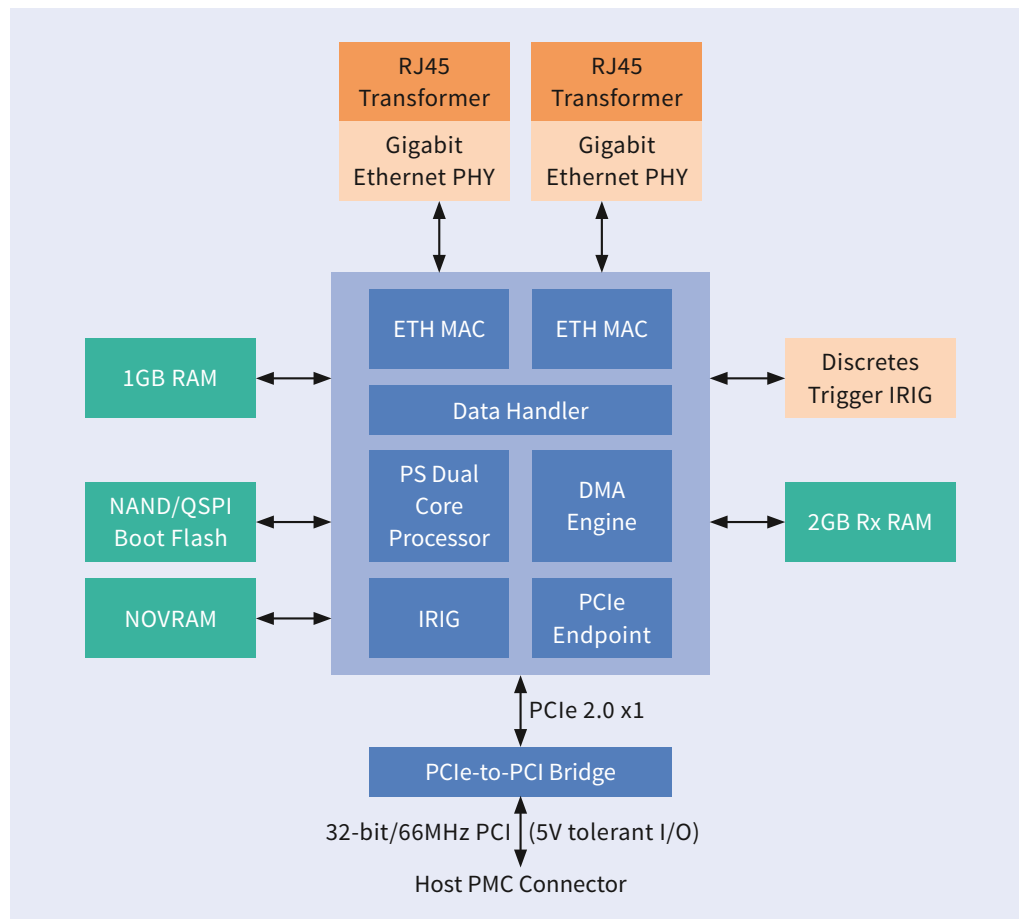
AMCX-FDX-2 Block Diagram
