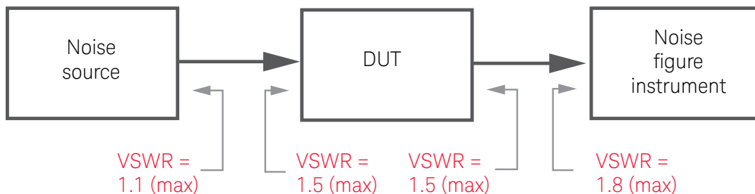
Figure 3-2. Example of mismatch effects.
