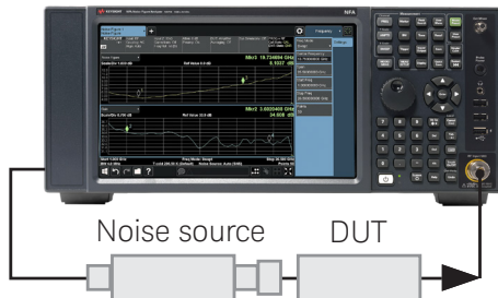
Figure 2-5. The Y-factor noise figure measurement requires two steps: (a) Calibration, (b) Measurement of DUT.
