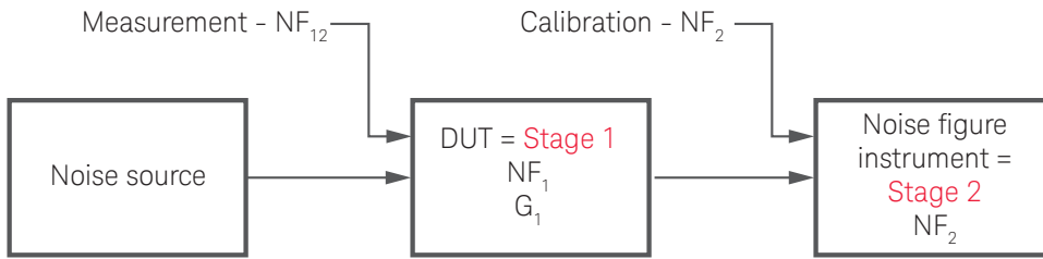
Figure 2-4. Noise figure measurement uses a two-stage system.
