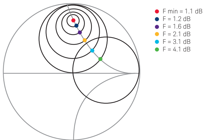
Figure 3-3 The noise figure of most devices depends on the input impedance presented to the device. Without full knowledge of the noise figure contours on a Smith chart, mismatch corrections can be uncertain and may introduce more error.
