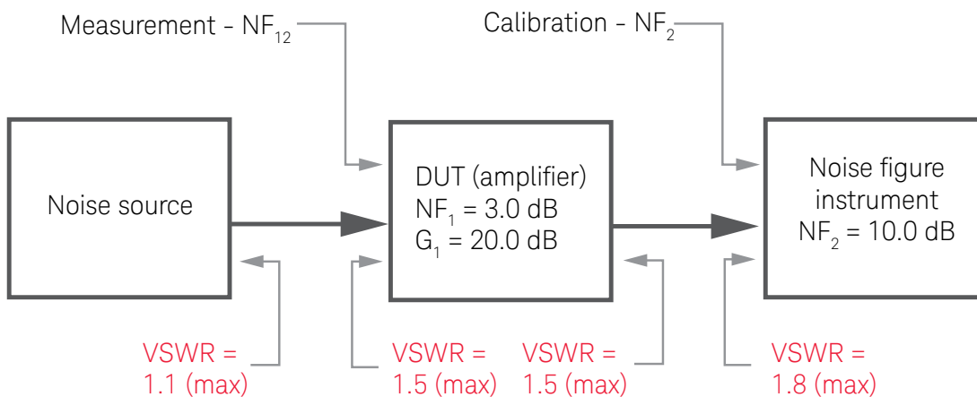
Figure 5-1 Model for uncertainty calculation.
