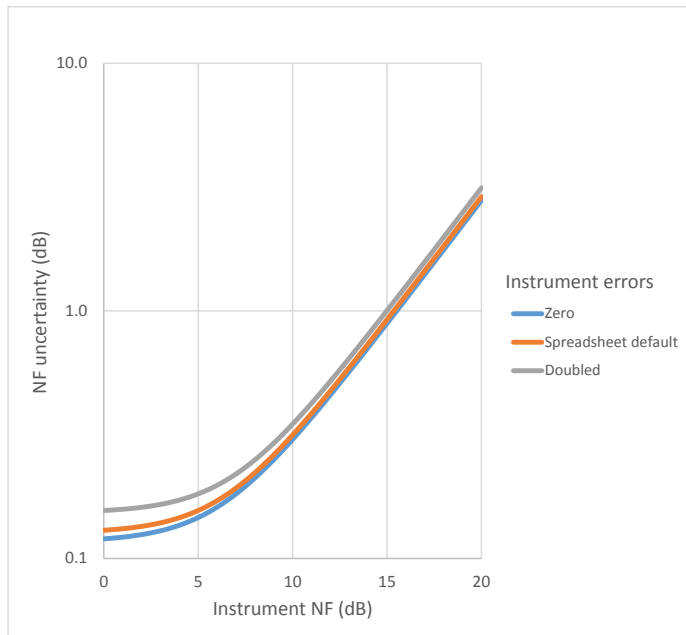
Figure 6-1. Uncertainty versus instrument NF and instrument errors (DUT gain 10 dB, other variables at default values used in spreadsheet).
