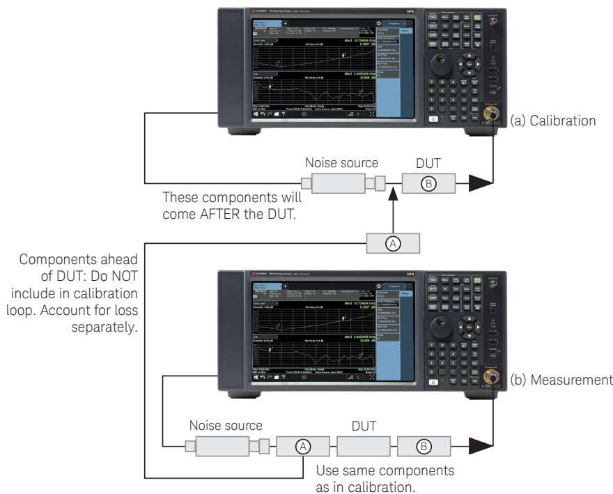
Figure 3-10. Components labeled B that are in the calibration loop (subfigure a) must come after the DUT during the measurement (subfigure b). Components between the noise source and the DUT input (labeled A) must not be included in the calibration loop.
