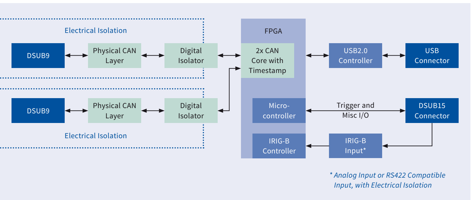
APU825 Block Diagram
