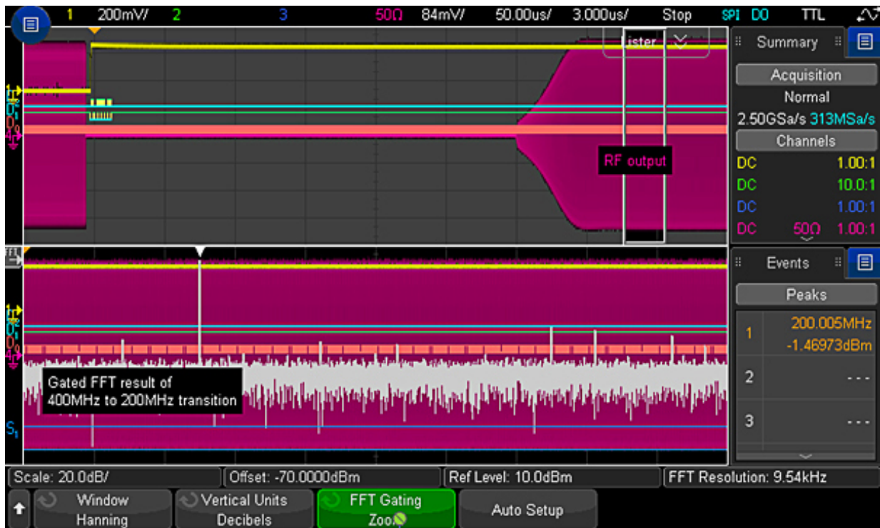
Figure 21d: RF signal settled down at 200 MH as indicated in the search lister.
