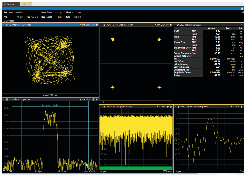
Analysis of a ZigBee signal with the R&S®VSE-K70.
