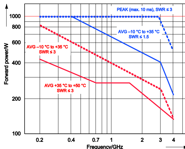
Power-handling capacity
