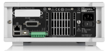
R&S®NGU201, rear view
