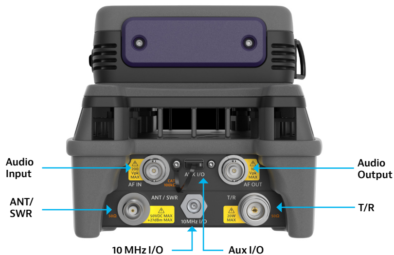
CX100 Top Input/Output Connectors
