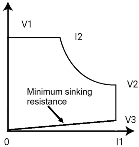
Figure 9. EL4900 characteristic
