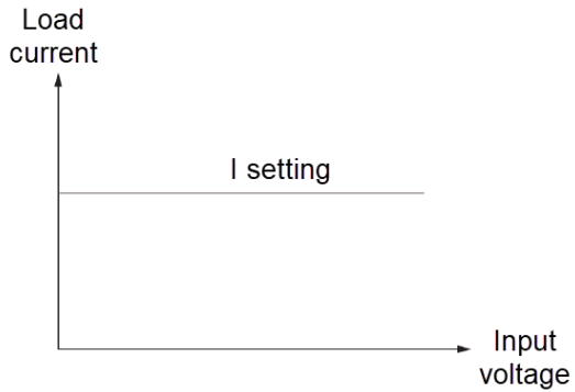
Current Priority (CC mode)
